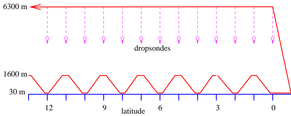
Figure 4: Trajectory of C-130 in 95° W missions. The nominal elevations for each flight segment are shown at left. Dropsondes were launched from 6300 m every degree from the equator to 12° N on the return segment.
