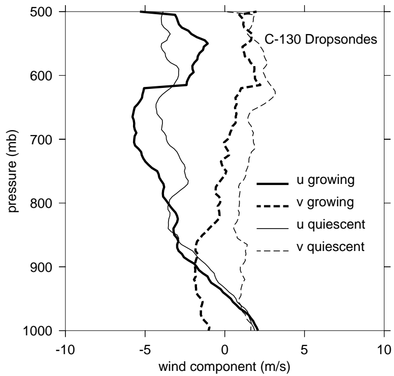
Figure 10: Wind profiles corresponding to the thermodynamic profiles shown in figure 9. Convectively developing cases are shown by thick lines and quiescent regions by thin lines.
