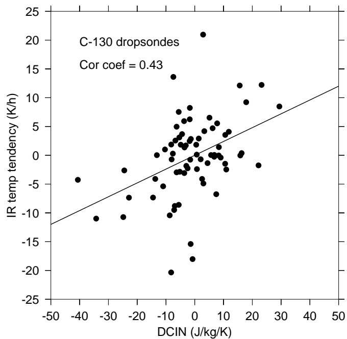
Figure 16: Scatter plot of DCIN for C-130 dropsondes in the ITCZ study region versus infrared brightness temperature tendency in a 0.4^\circ \times 0.4^\circ box centered on each dropsonde.
