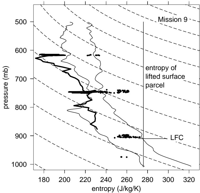
Figure 15: As in figure 11 except for a region of convection capped by a dry layer near 96.5^{\circ} W, 11^{\circ} N on 20 September 2001 (mission 9; day 263). The thin lines represent an aircraft sounding taken a few tens of kilometers north of the convection. The thick line is the entropy in the immediate vicinity of the convection.
