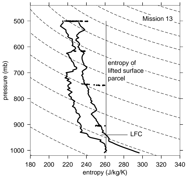
Figure 11: Proximity sounding showing entropy and saturated entropy profiles in inflow region for a weak convective line near 95^{\circ} W, 12^{\circ} N on 29 September 2001 (mission 13; day 272). The dots show one second samples of the in-cloud entropy (cloud water density > 0.05 \text{ g m}^{-3} , updraft > 1 \text{ m s}^{-1} ) measured during C-130 penetrations at various levels.
