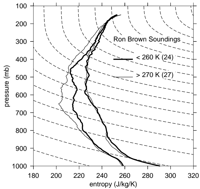
Figure 20: Respective averages of Ron Brown soundings for mean infrared brightness temperatures in the ITCZ study region less than 260 K and greater than 270 K. The numbers in parentheses give the number of soundings in each average.
