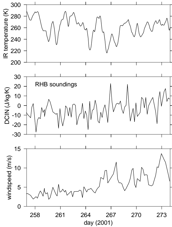
Figure 17: Satellite infrared brightness temperature over the ITCZ study region (upper panel), DCIN (middle panel) and wind speed averaged over the lowest 100 mb (lower panel) for 17 d of ship Ron Brown radiosonde soundings taken near 95^\circ W, 10^\circ N.
