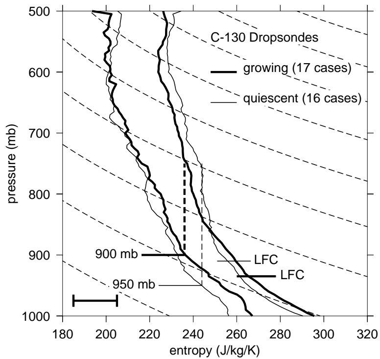
Figure 9: As in figure 8 except soundings in convectively developing (thick lines) and quiescent regions (thin lines). The vertical dashed lines show the origins of lifted parcels in each case which would be neutrally buoyant at 750 mb.
