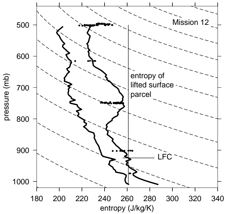
Figure 14: As in figure 11 except for a region of very weak convection reaching the middle troposphere near 94^{\circ} W, 9^{\circ} N on 28 September 2001 (mission 12; day 271).
