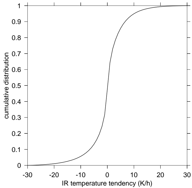
Figure 7: Cumulative distribution of infrared brightness temperature tendencies over the ITCZ study region during the EPIC2001 field program.
