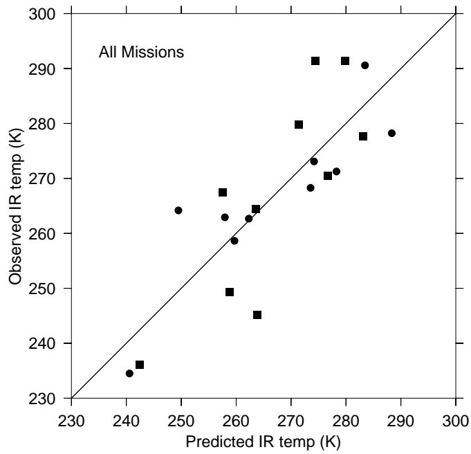
Figure 19: Observed versus predicted infrared brightness temperature for all 20 EPIC2001 missions. The circles represent missions using C-130 dropsondes while the boxes represent those using P-3 dropsondes. The correlation coefficient is 0.82 and the correlation is significant at the 99% level.
