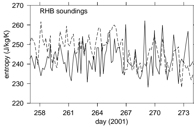
Figure 18: Threshold entropy s_t (saturated entropy averaged over 810 – 830 mb; solid line) and boundary layer entropy s_b (entropy averaged over 900 – 1000 mb; dashed line) for Ron Brown soundings as shown in figure 17.
