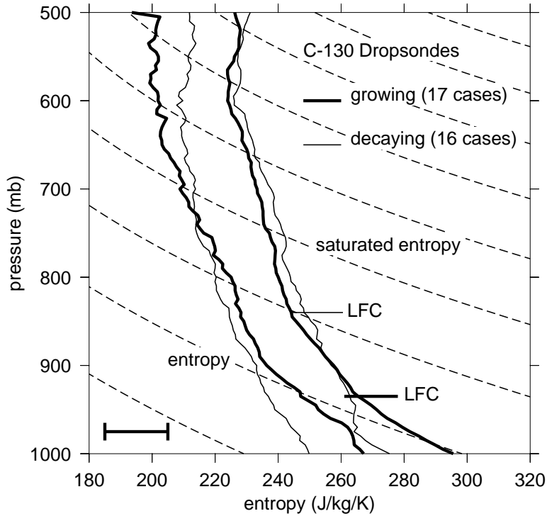
Figure 8: C-130 dropsonde soundings expressed as plots of entropy (left) and saturated entropy (right) versus pressure. The thick lines represent the average of soundings for which the satellite infrared brightness temperature is decreasing by more than 4 \text{ K h}^{-1} , whereas the thin lines are an average for which the brightness temperature is increasing by more than this rate. The levels of free convection (LFC) of surface parcels are indicated for the two cases. The dashed lines represent contours of constant potential temperature at 5 K intervals. Note that the entropy is conserved in ascent and descent by both saturated and unsaturated parcels, whereas the saturated entropy of an unsaturated parcel is not conserved, but moves along a potential temperature contour in ascent and descent. The error bar in the lower left corner shows the typical standard deviation of both the entropy and the saturated entropy at each level.
