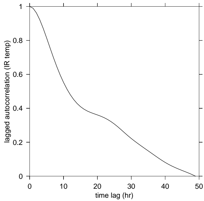
Figure 6: Lagged autocorrelation function over the period of the field program for the satellite infrared brightness temperature averaged over the 4^\circ \times 4^\circ ITCZ study region.
