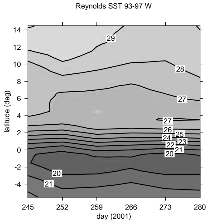
Figure 2: Reynolds SST in degrees Celsius as a function of latitude and time during the EPIC2001 project, averaged from 93° W to 97° W.
