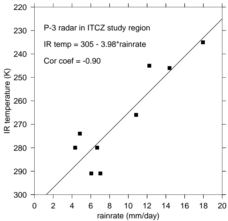
Figure 5: Plot of rainfall rate from the P-3 radar averaged over the ITCZ study region vs. the average infrared brightness temperature over this region.
