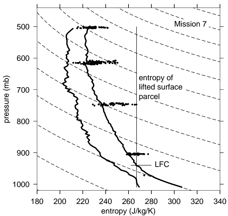
Figure 12: As in figure 11 except for a region of growing convective cells in low shear near 95^\circ W, 11.5^\circ N on 16 September 2001 (mission 7; day 259).
