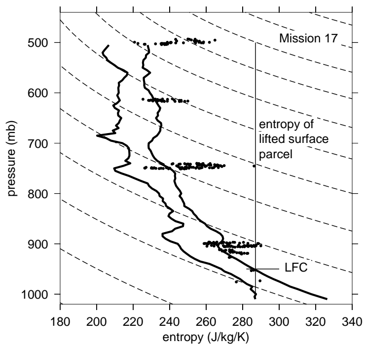
Figure 13: As in figure 11 except for a region of vigorous growing convection in easterly shear near 94^{\circ} W, 12^{\circ} N on 6 October 2001 (mission 17; day 279).
