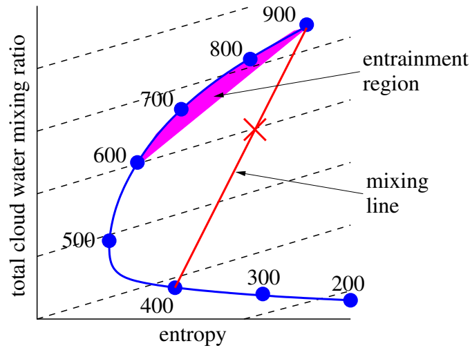
Figure 4.6: Atmospheric sounding represented by labeled curve, with labels being pressure in hPa. The solid straight line is a mixing line between 400 hPa and 900 hPa (see text) and the dashed lines are contours of constant potential temperature. The cross indicates the characteristics of the mixture which has potential temperature equal to the environmental potential temperature at 600 hPa. The shaded region indicates possible values of cloud water mixing ratio and entropy in the cloud at 600 hPa that could result from entrainment between 600 hPa and 900 hPa.
